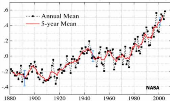
(a) Global-Mean Surface Temperature Anomaly (°C)
